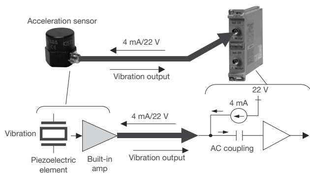
Connecting a built-in amp type acceleration sensor
